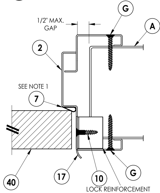
4 3 HORIZONTAL CROSS SECTION Steel Stud Installation
