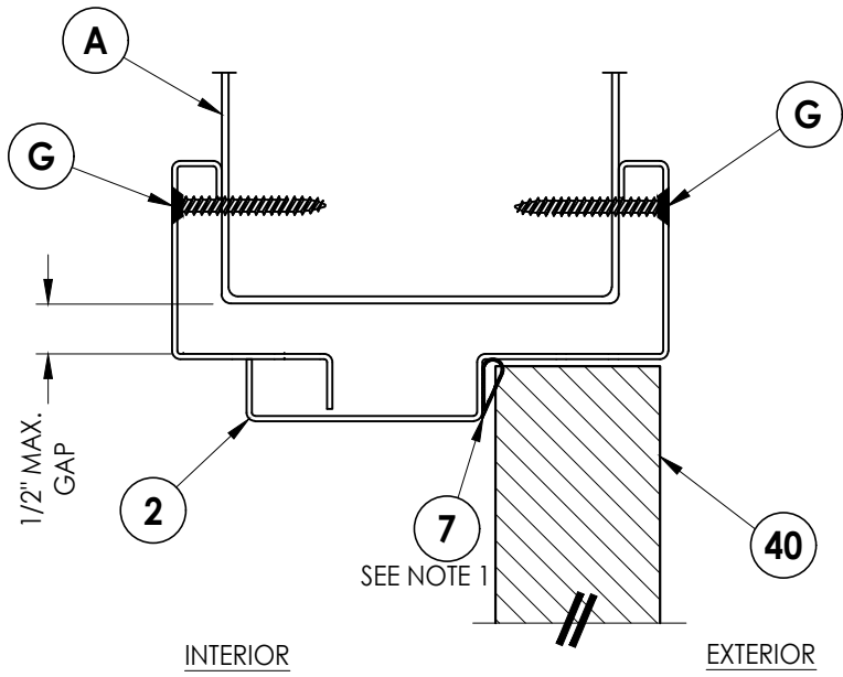
2 4 VERTICAL CROSS SECTION
