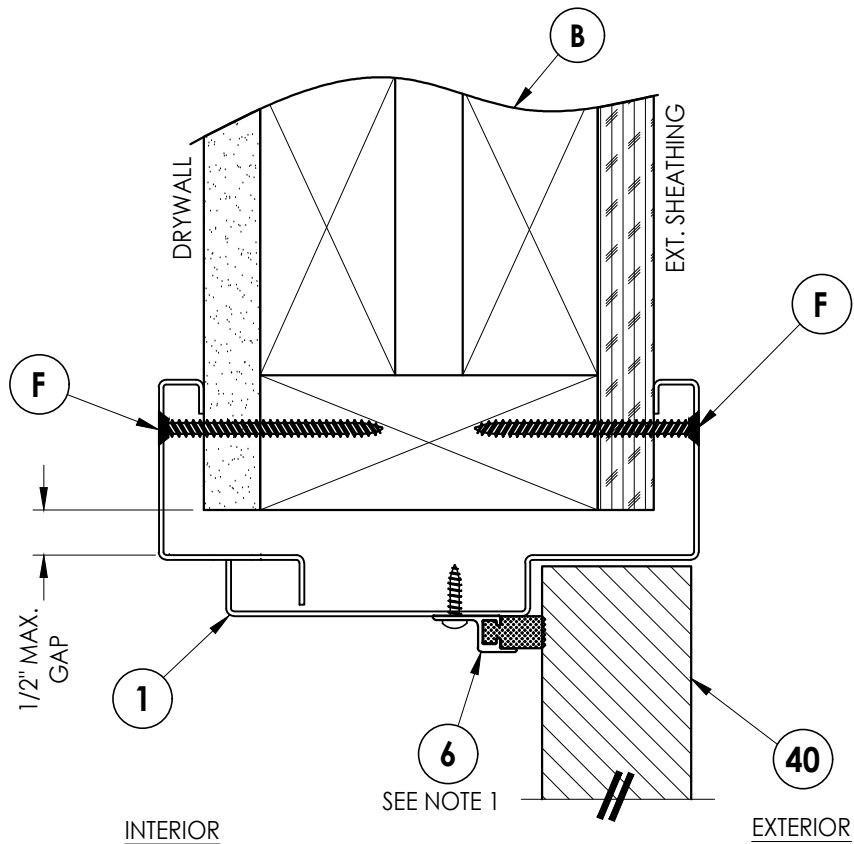
1 4 VERTICAL CROSS SECTION
