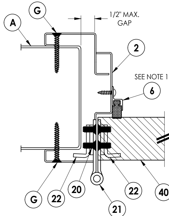
3 3 HORIZONTAL CROSS SECTION Steel Stud Installation
