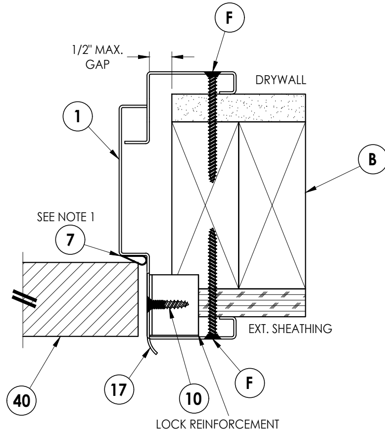
2 3 HORIZONTAL CROSS SECTION Wood Stud Installation
