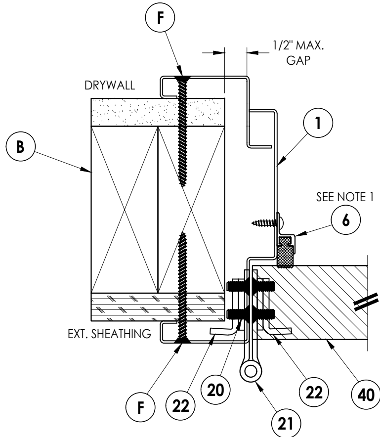
1 3 HORIZONTAL CROSS SECTION Wood Stud Installation
